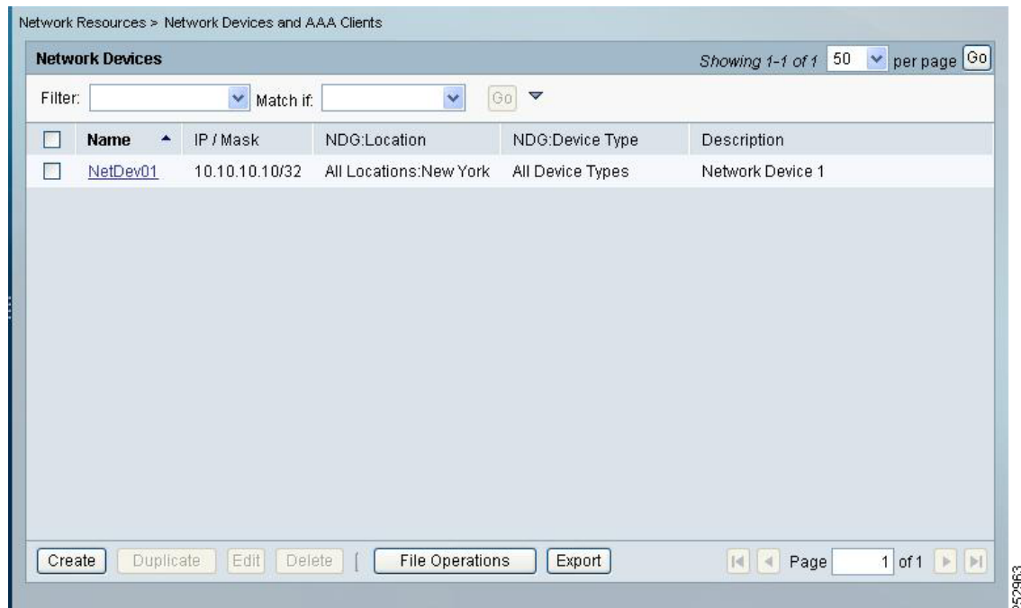
Figure 5-5 List Page
